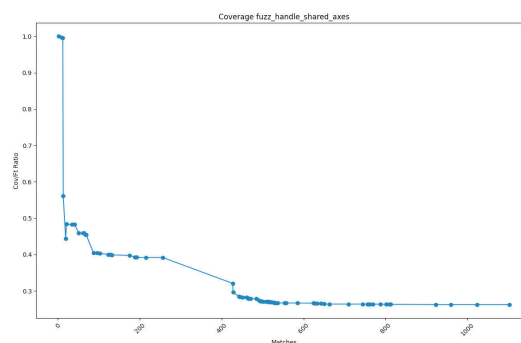
Figure 1: Example of a good fuzz target generated by LLM (handle-shared-axes-fuzz)
