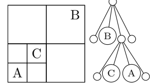
Inserting B: Subdivide, shift A, Inserting C: Subdivide, shift A, shift B from root
